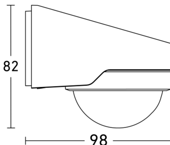
Dimension Drawing 2
